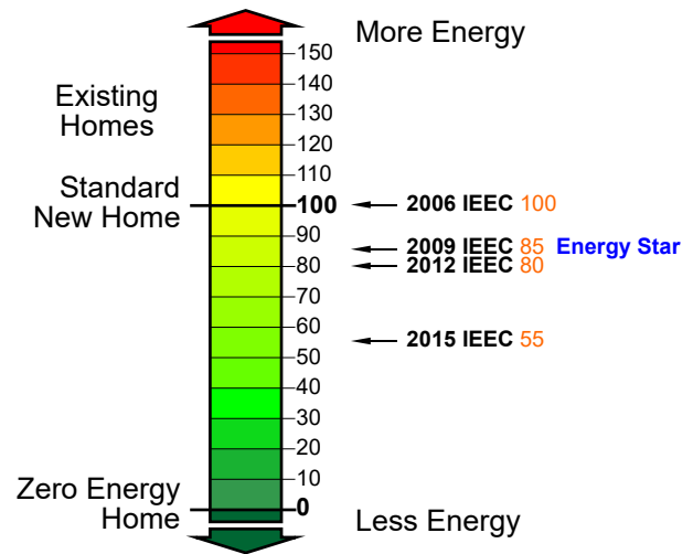
Figure 3 HERS Index and IECC Code Requirements
