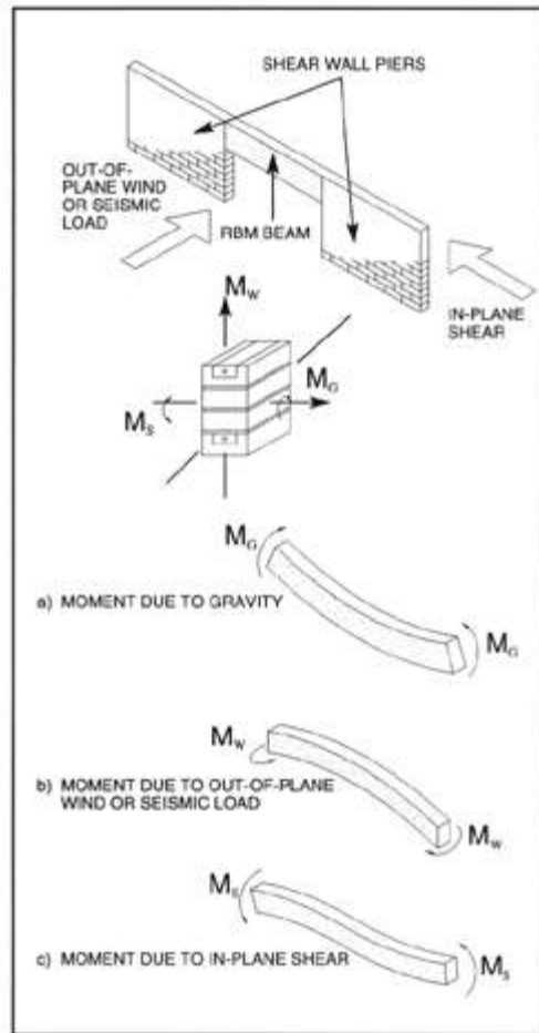
Moments on RBM Beam FIG. 2
