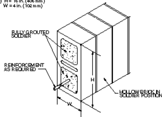
Design Curves for Soldier Course Beams FIG. 6
