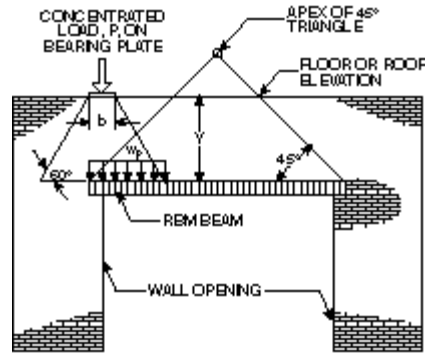
Loads on RBM Beam FIG. 4
