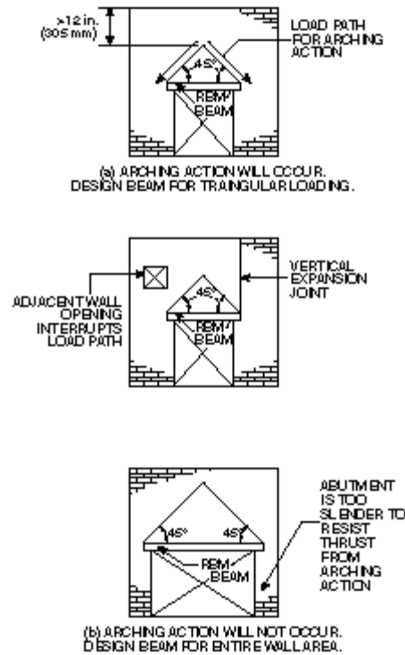
Conditions for Arching Action FIG. 3
