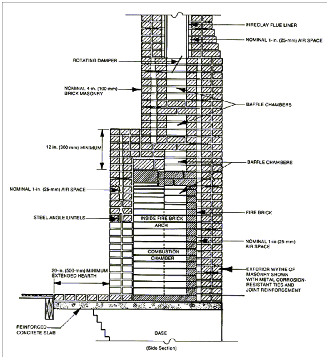
Modified Conventional Fireplace
