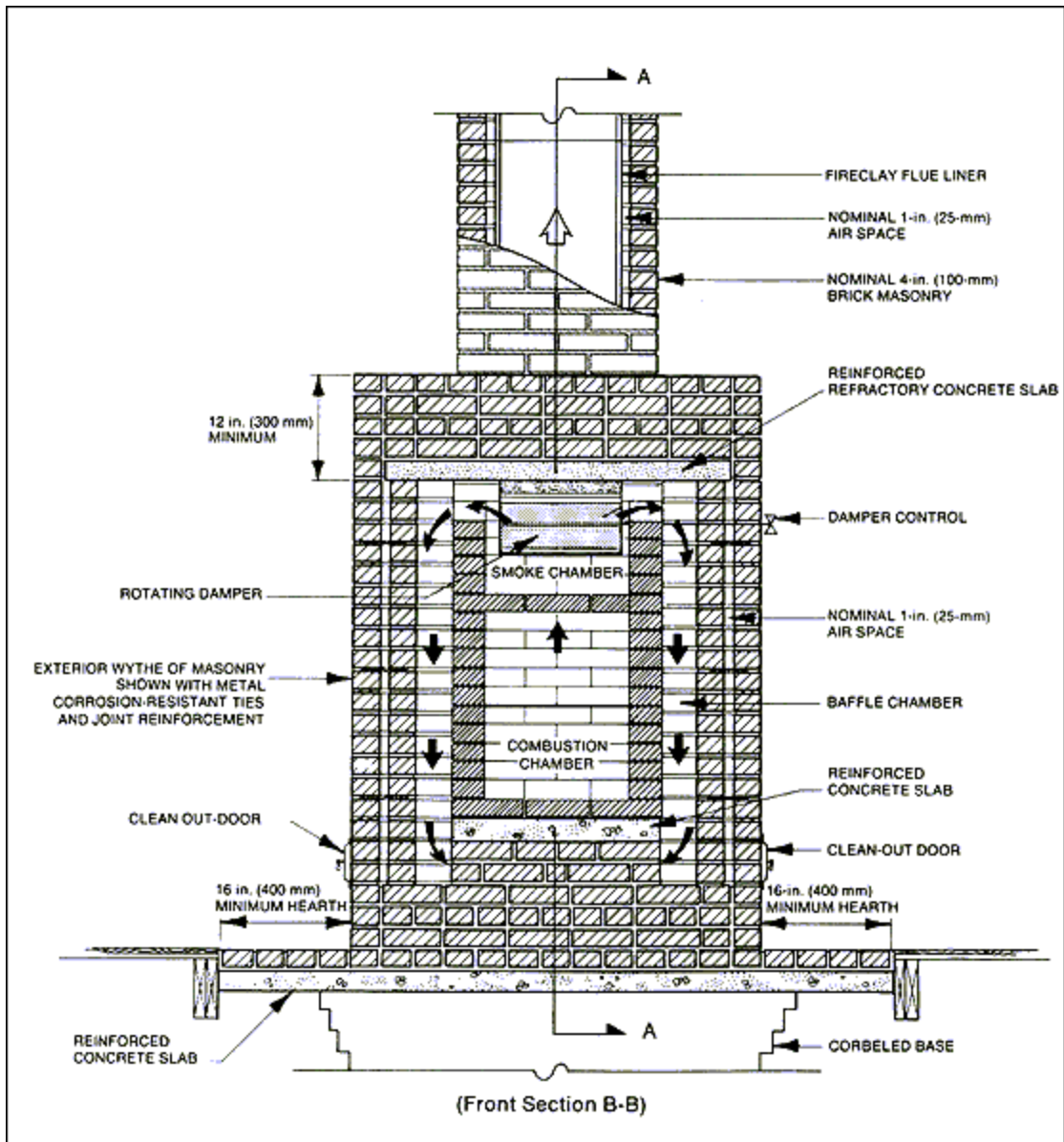
Fountain-Style Brick Masonry Heater
