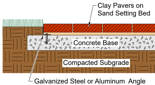
(e) Steel Angle Edge Restraint
